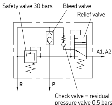
Relief valve circuit diagram
